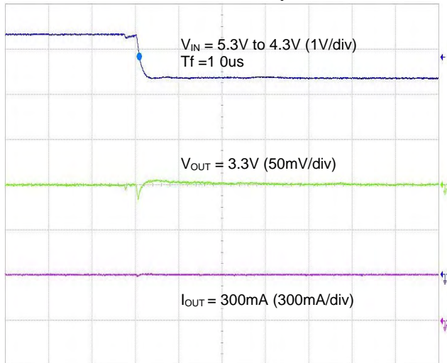
Time (50us/div)
