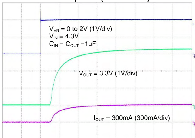
Time (50us/div)
