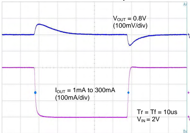
Time (100us/div)
