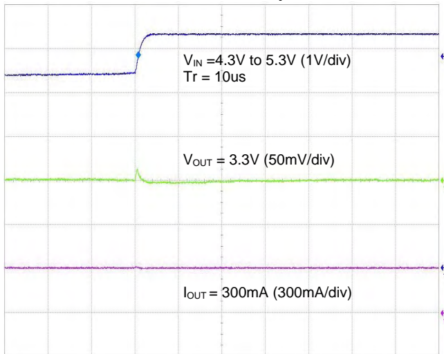
Time (50us/div)
